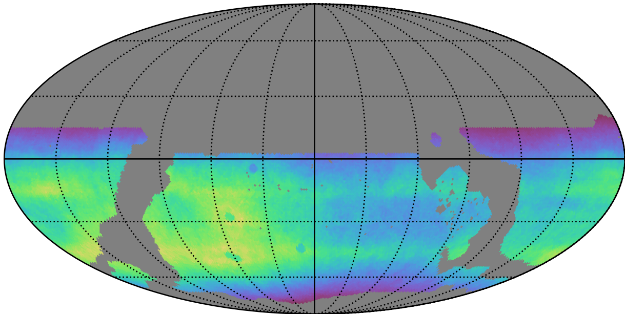
ddf_loaded_fl2_v3.4_10yrs WFD all bands: Normalized Teff
