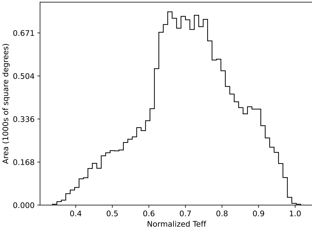
ddf_loaded_fl2_v3.4_10yrs WFD all bands: Normalized Teff
