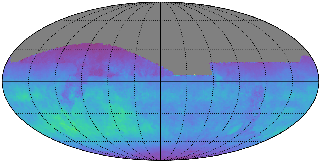
ddf_loaded_fl2_v3.4_10yrs All sky z band: Normalized Teff
