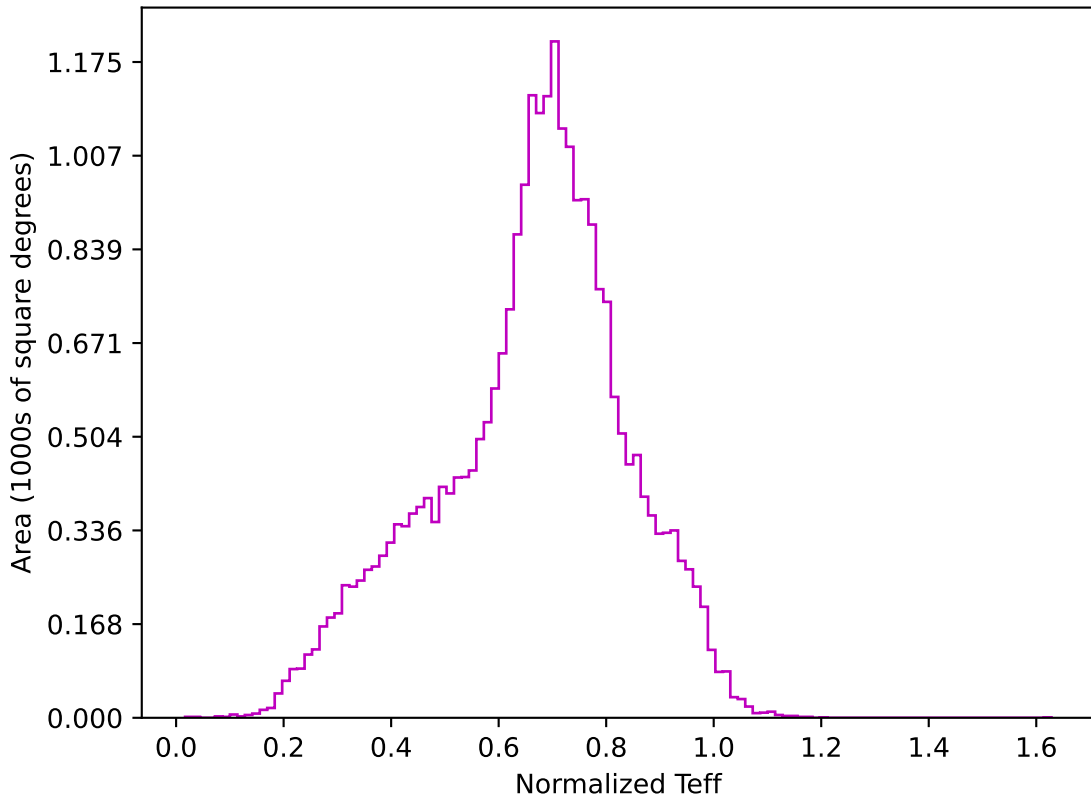
ddf_loaded_fl2_v3.4_10yrs All sky z band: Normalized Teff
