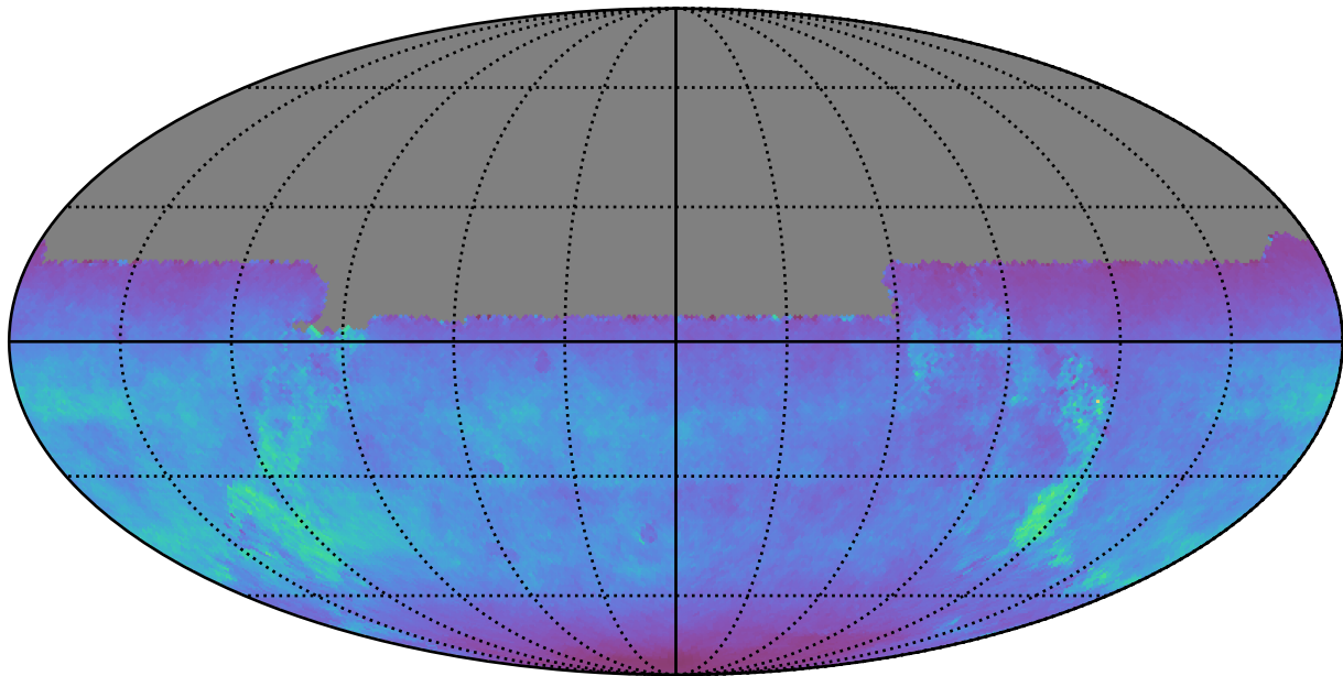
ddf_loaded_fl2_v3.4_10yrs All sky u band: Normalized Teff
