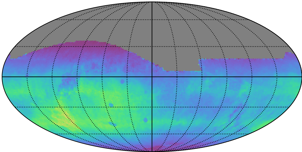
ddf_loaded_fl2_v3.4_10yrs All sky r band: Normalized Teff
