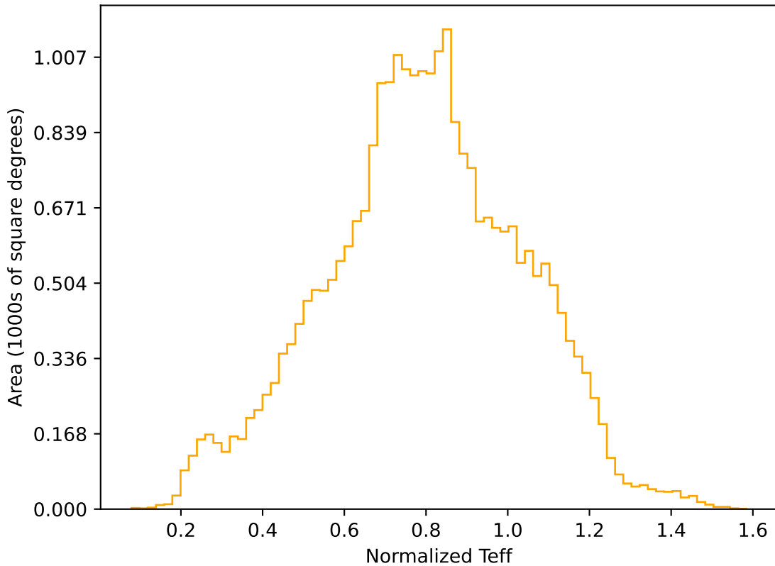
ddf_loaded_fl2_v3.4_10yrs All sky r band: Normalized Teff
