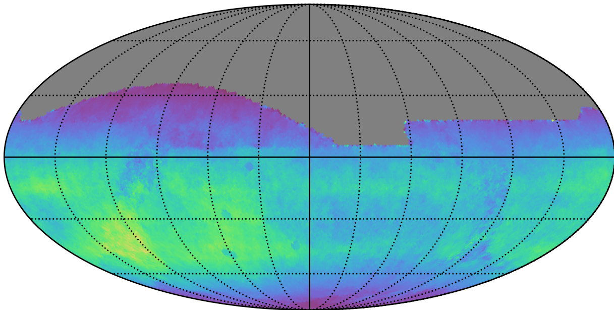
ddf_loaded_fl2_v3.4_10yrs All sky i band: Normalized Teff
