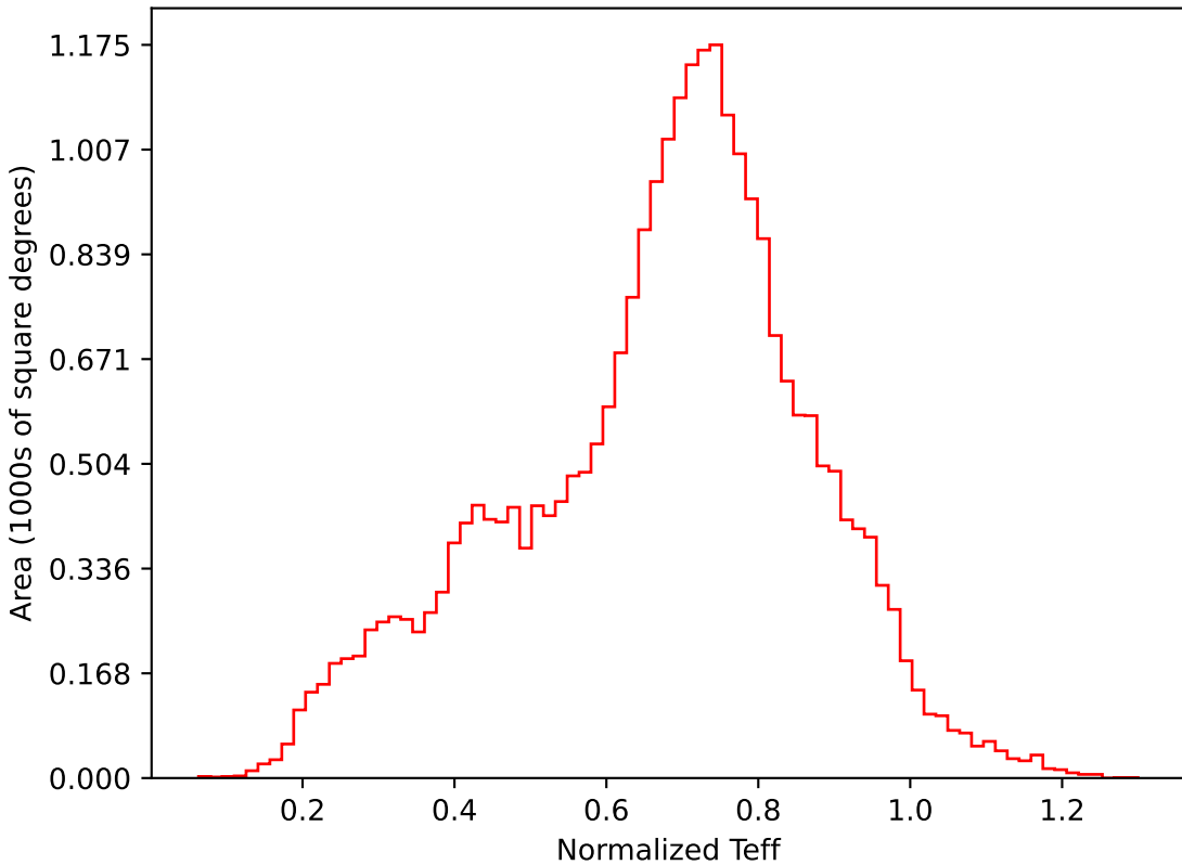
ddf_loaded_fl2_v3.4_10yrs All sky i band: Normalized Teff
