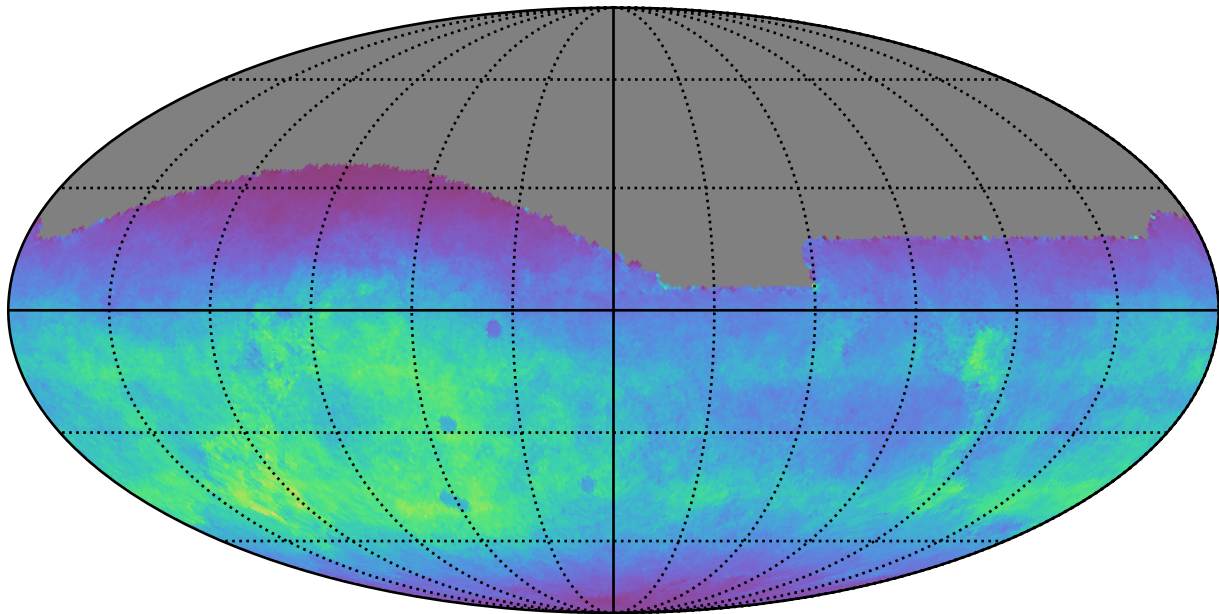
ddf_loaded_fl2_v3.4_10yrs All sky g band: Normalized Teff
