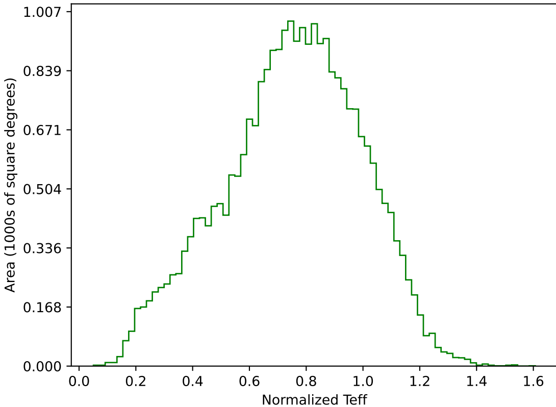
ddf_loaded_fl2_v3.4_10yrs All sky g band: Normalized Teff
