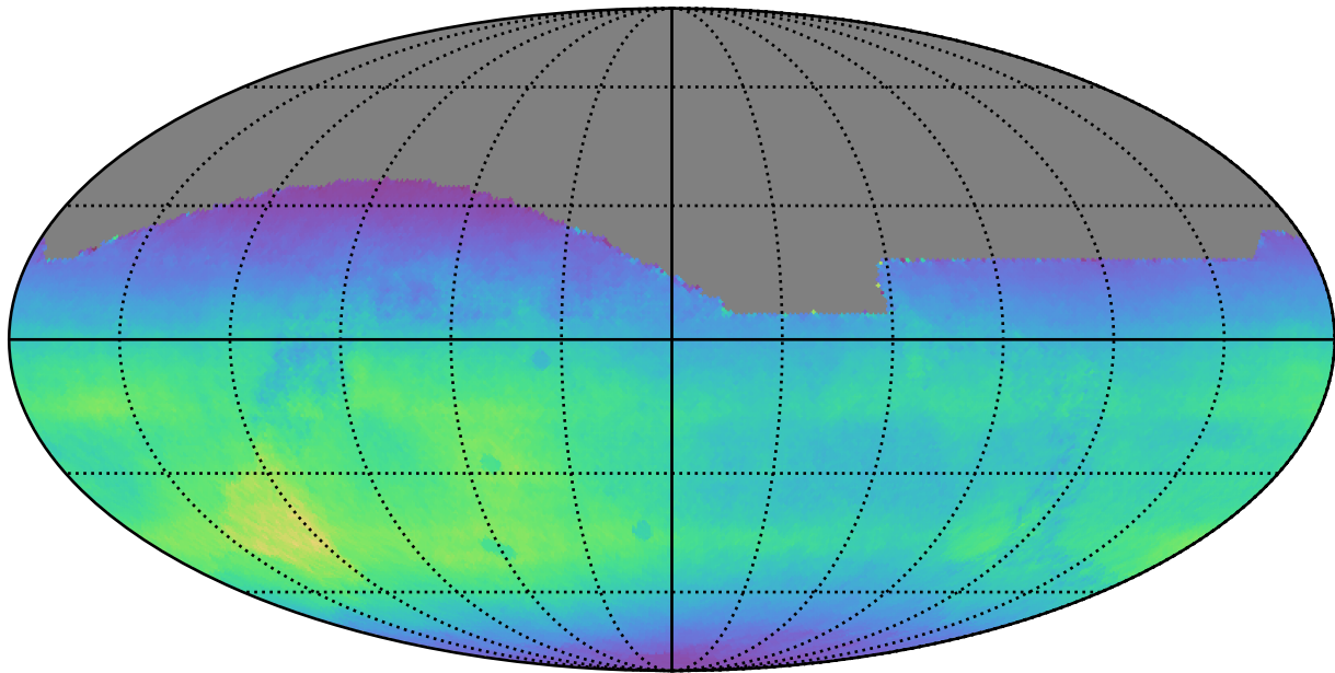
ddf_loaded_fl2_v3.4_10yrs All sky all bands: Normalized Teff
