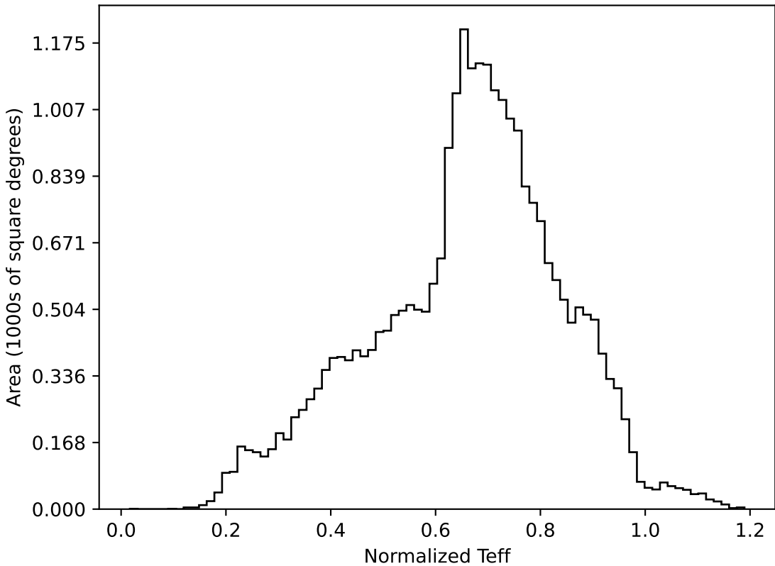
ddf_loaded_fl2_v3.4_10yrs All sky all bands: Normalized Teff
