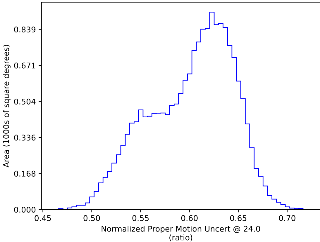
ddf_loaded_fl2_v3.4_10yrs WFD: Normalized Proper Motion Uncert @ 24.0
