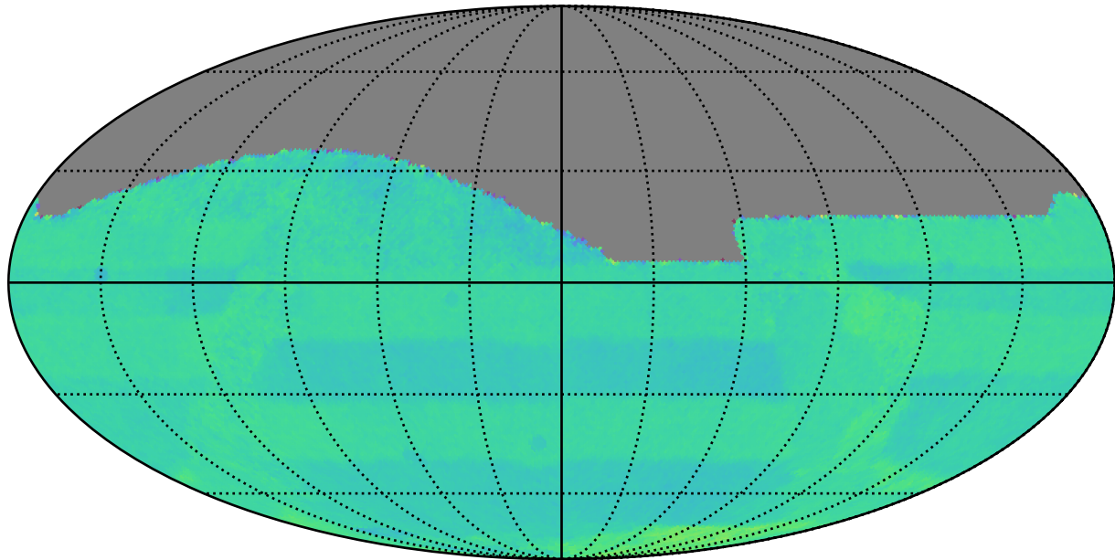
ddf_loaded_fl2_v3.4_10yrs All sky: Normalized Proper Motion Uncert @ 20.5
