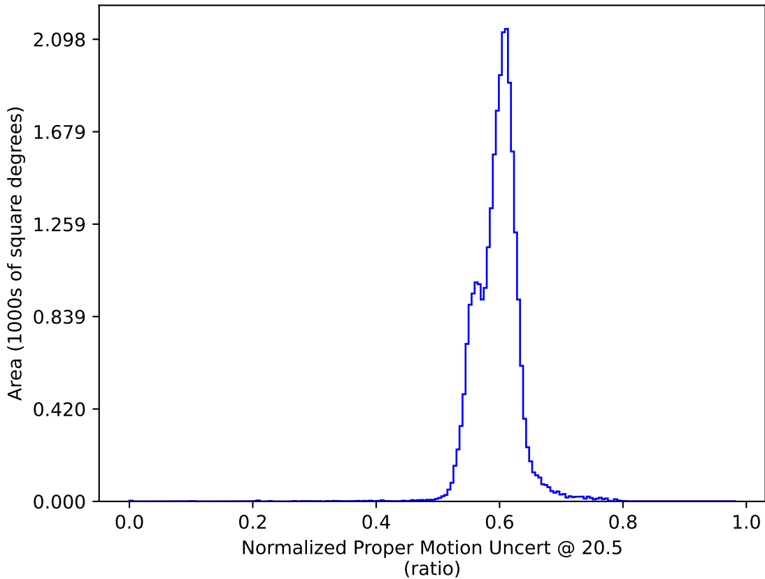
ddf_loaded_fl2_v3.4_10yrs All sky: Normalized Proper Motion Uncert @ 20.5
