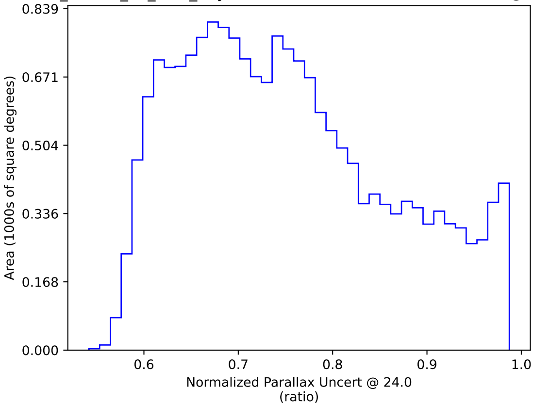
ddf_loaded_fl2_v3.4_10yrs WFD: Normalized Parallax Uncert @ 24.0
