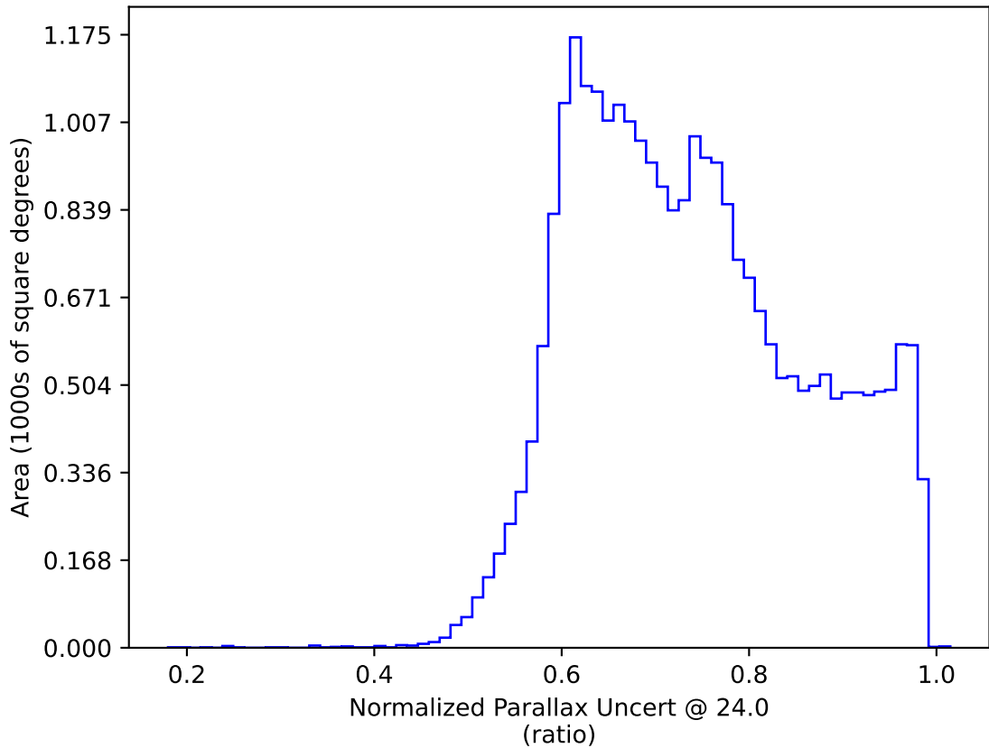
ddf_loaded_fl2_v3.4_10yrs All sky: Normalized Parallax Uncert @ 24.0
