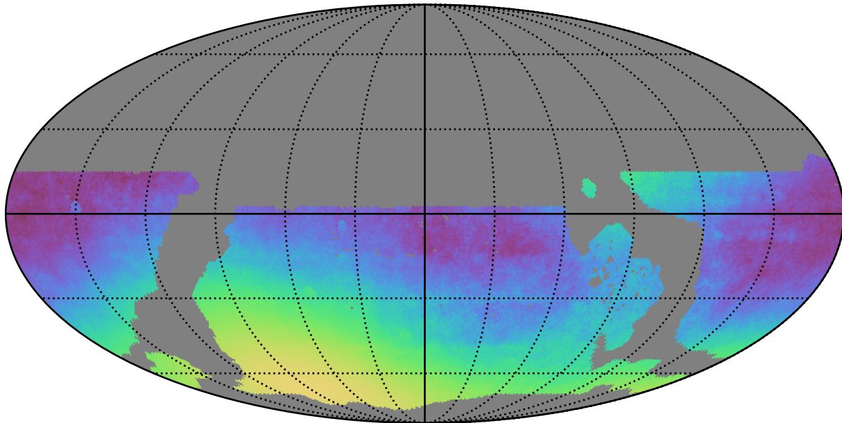
ddf_loaded_fl2_v3.4_10yrs WFD: Normalized Parallax Uncert @ 22.4
