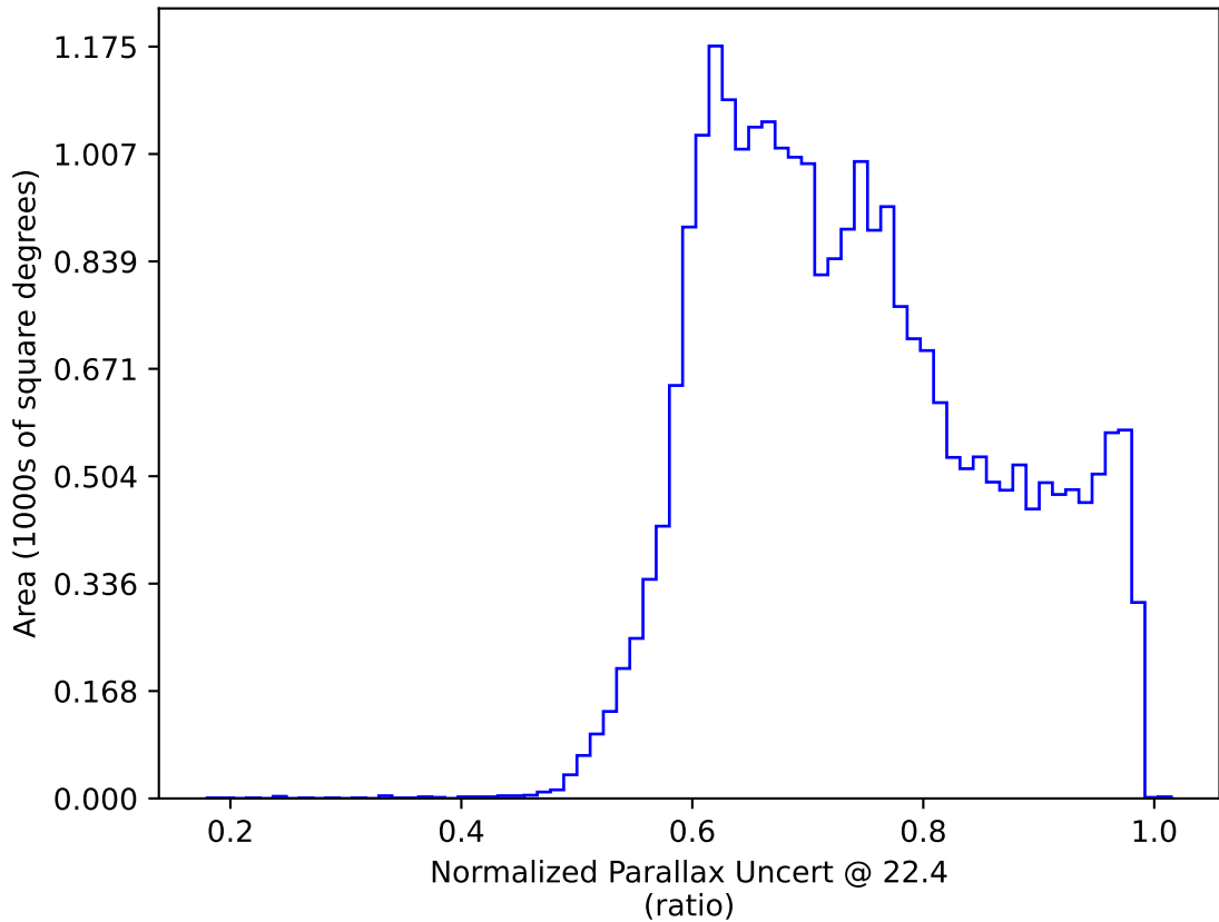
ddf_loaded_fl2_v3.4_10yrs All sky: Normalized Parallax Uncert @ 22.4
