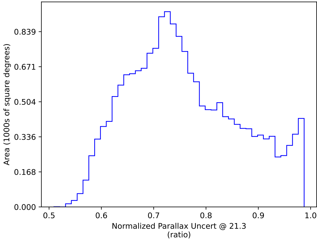
ddf_loaded_fl2_v3.4_10yrs WFD y band only: Normalized Parallax Uncert @ 21.3
