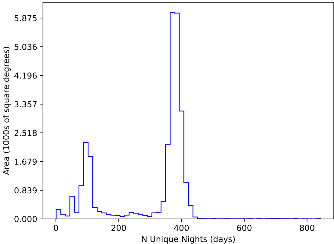
ddf_loaded_fl2_v3.4_10yrs All sky all bands: N Unique Nights
