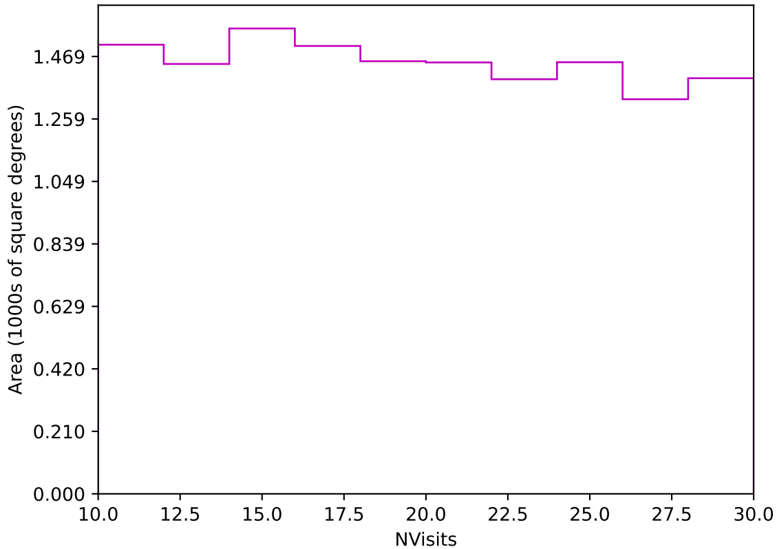
ddf_loaded_fl2_v3.4_10yrs Yr 3-4 z band: NVisits
