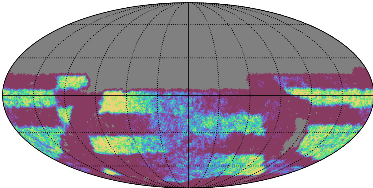
ddf_loaded_fl2_v3.4_10yrs Yr 3-4 y band: NVisits
