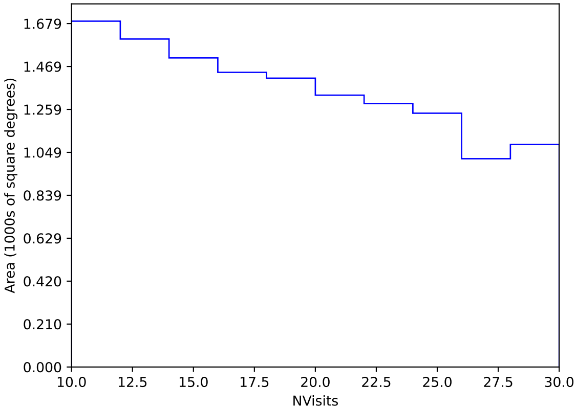
ddf_loaded_fl2_v3.4_10yrs Yr 3-4 y band: NVisits
