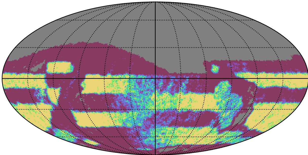
ddf_loaded_fl2_v3.4_10yrs Yr 3-4 r band: NVisits
