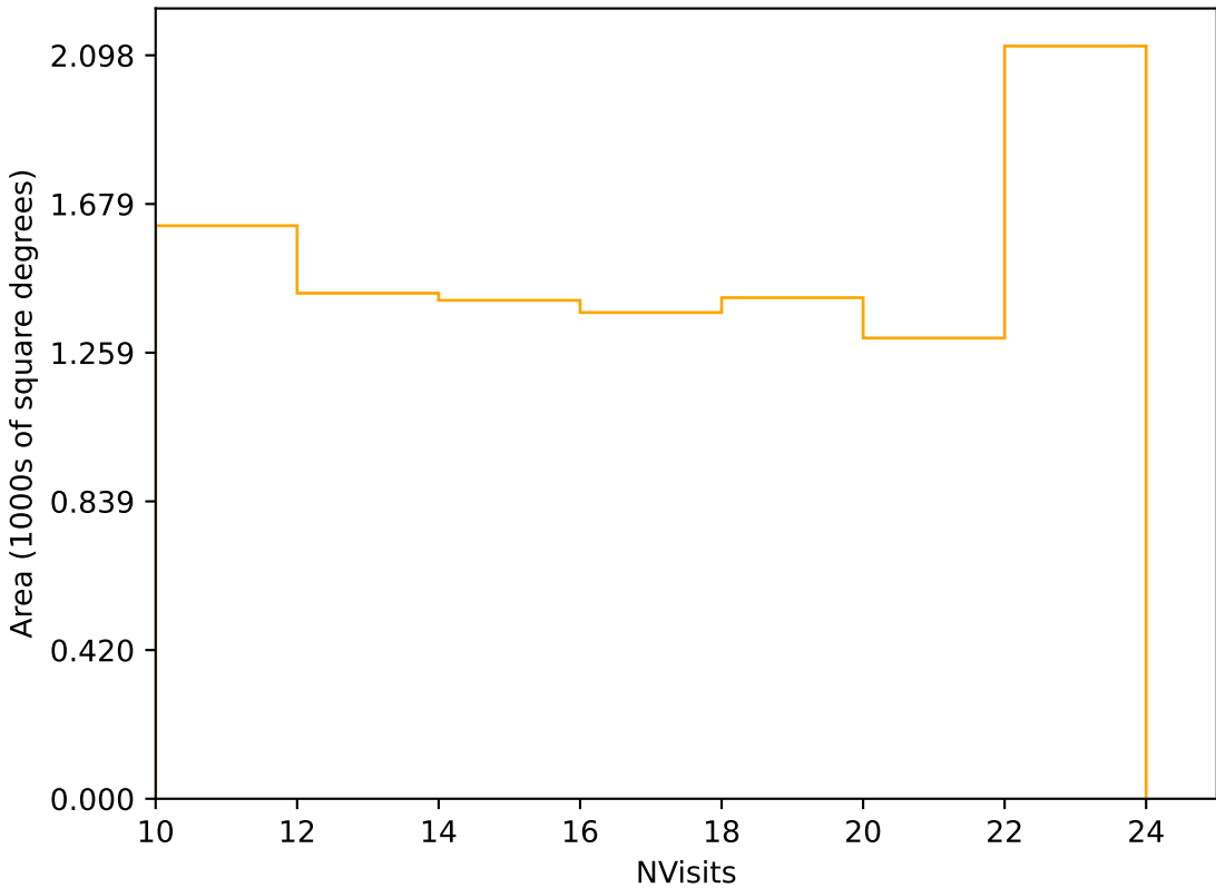
ddf_loaded_fl2_v3.4_10yrs Yr 3-4 r band: NVisits
