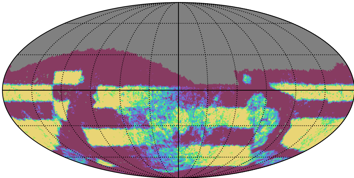
ddf_loaded_fl2_v3.4_10yrs Yr 3-4 i band: NVisits
