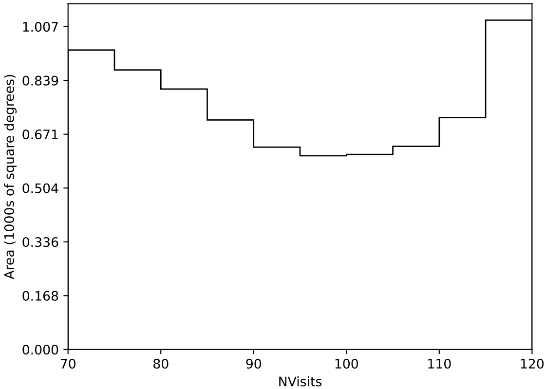
ddf_loaded_fl2_v3.4_10yrs Yr 3-4 all bands: NVisits
