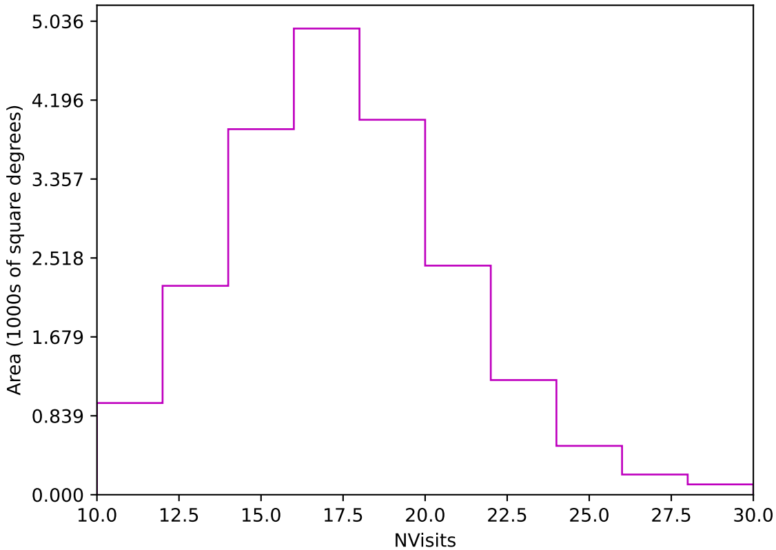
ddf_loaded_fl2_v3.4_10yrs Yr 1 z band: NVisits
