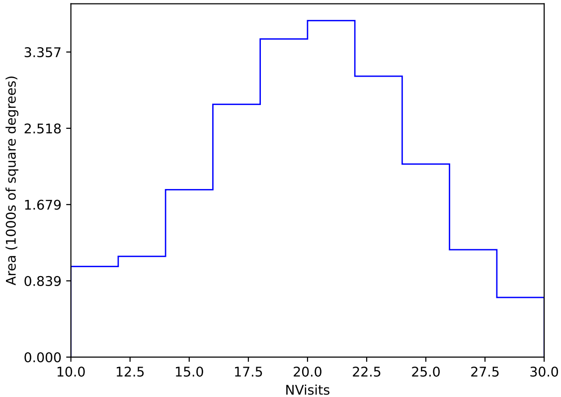
ddf_loaded_fl2_v3.4_10yrs Yr 1 y band: NVisits
