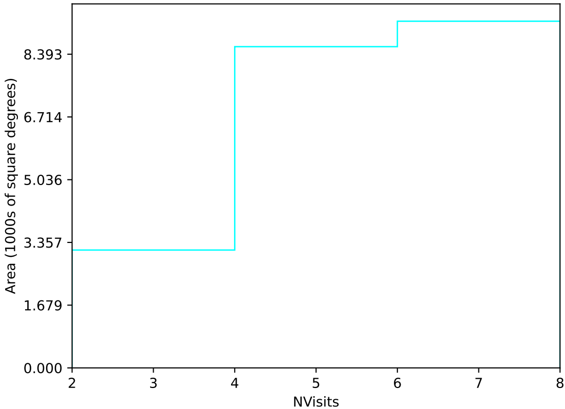
ddf_loaded_fl2_v3.4_10yrs Yr 1 u band: NVisits
