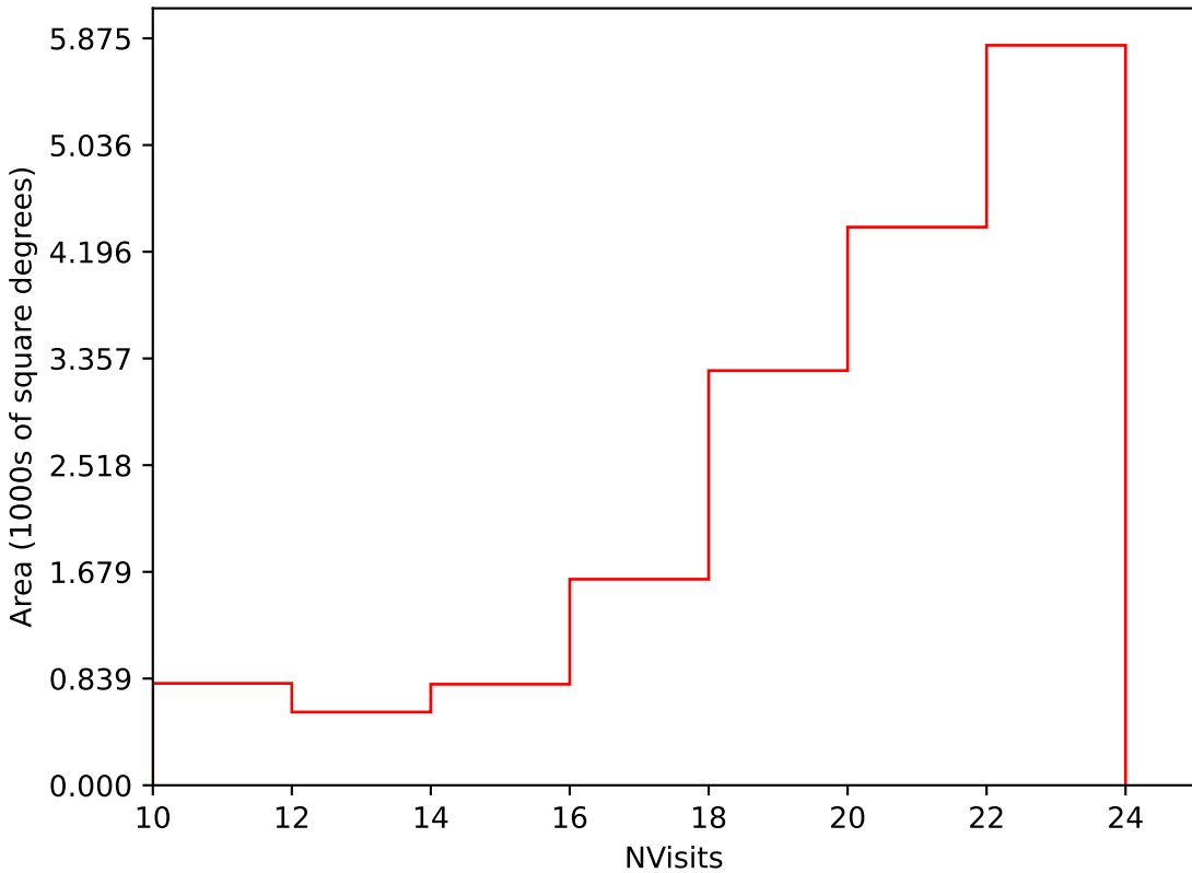
ddf_loaded_fl2_v3.4_10yrs Yr 1 i band: NVisits
