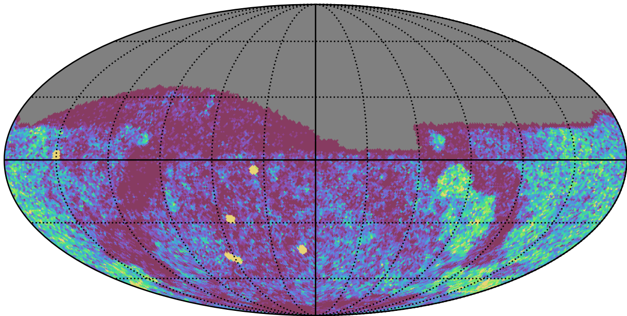
ddf_loaded_fl2_v3.4_10yrs Yr 1 g band: NVisits
