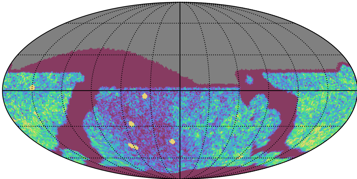
ddf_loaded_fl2_v3.4_10yrs Yr 1 all bands: NVisits
