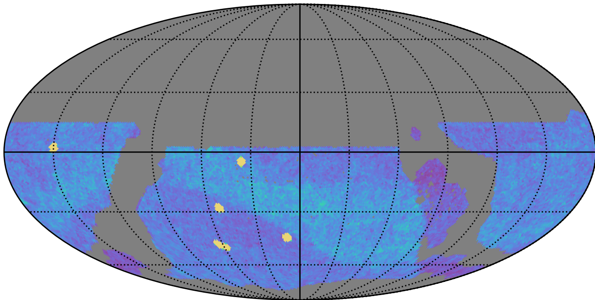
ddf_loaded_fl2_v3.4_10yrs WFD z band: NVisits
