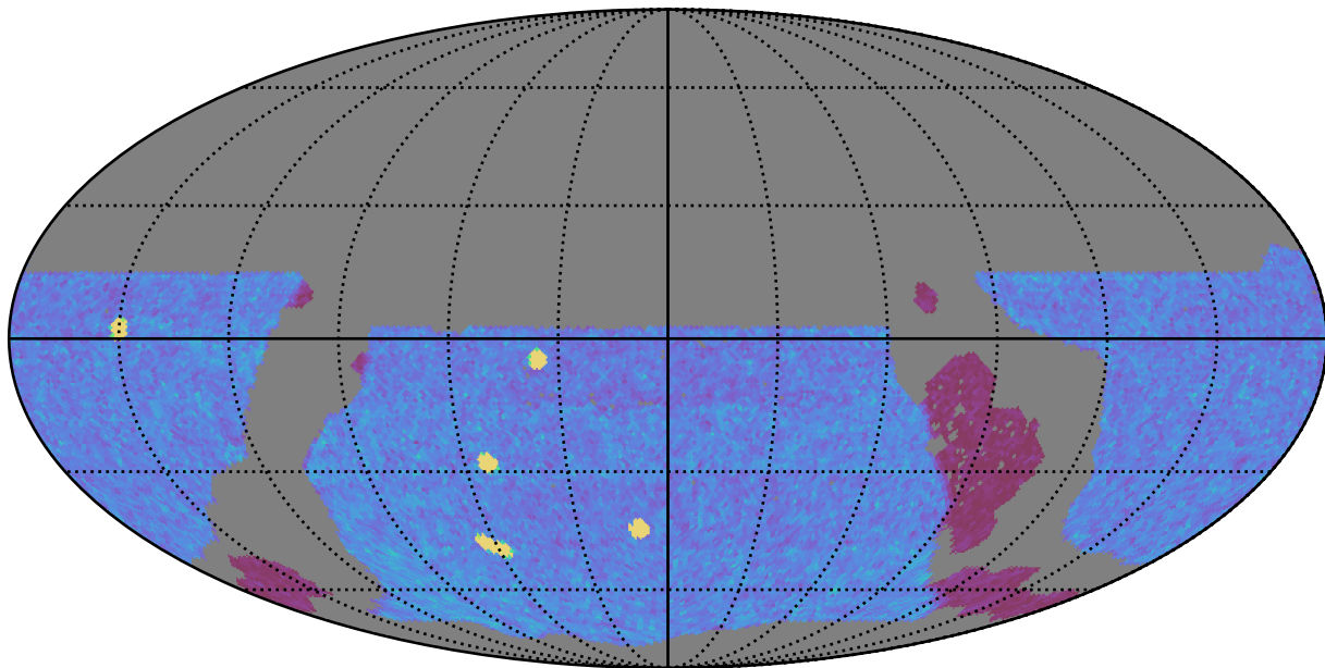
ddf_loaded_fl2_v3.4_10yrs WFD y band: NVisits
