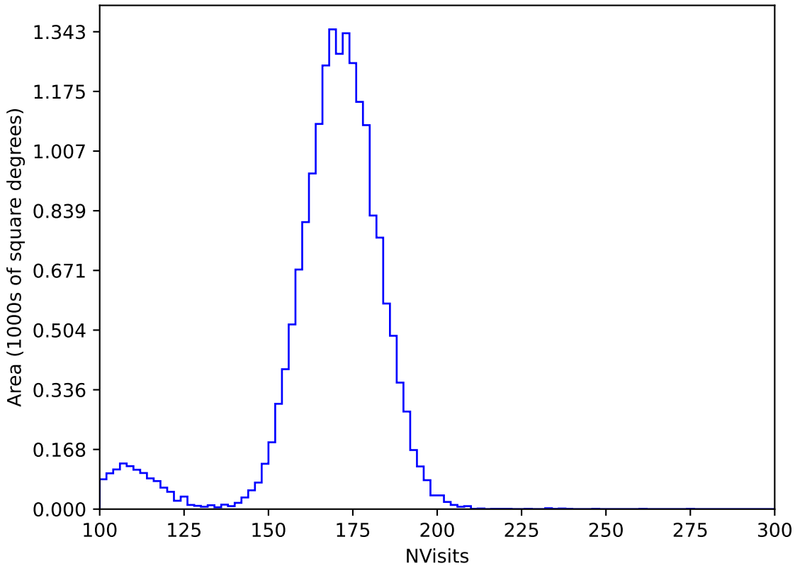
ddf_loaded_fl2_v3.4_10yrs WFD y band: NVisits
