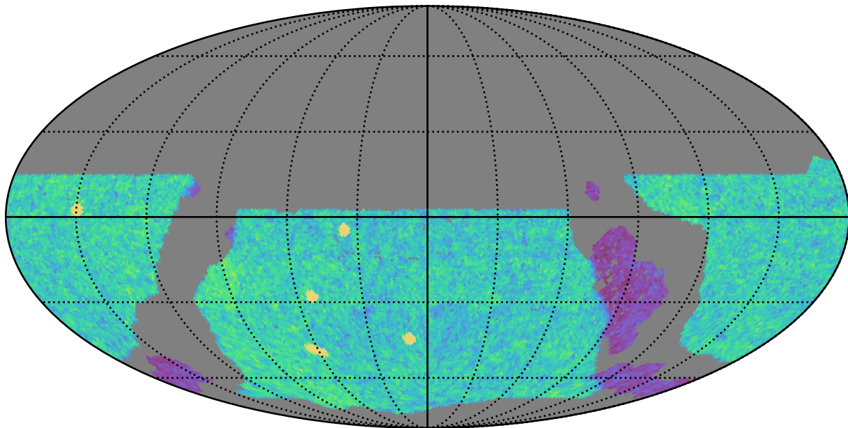
ddf_loaded_fl2_v3.4_10yrs WFD u band: NVisits
