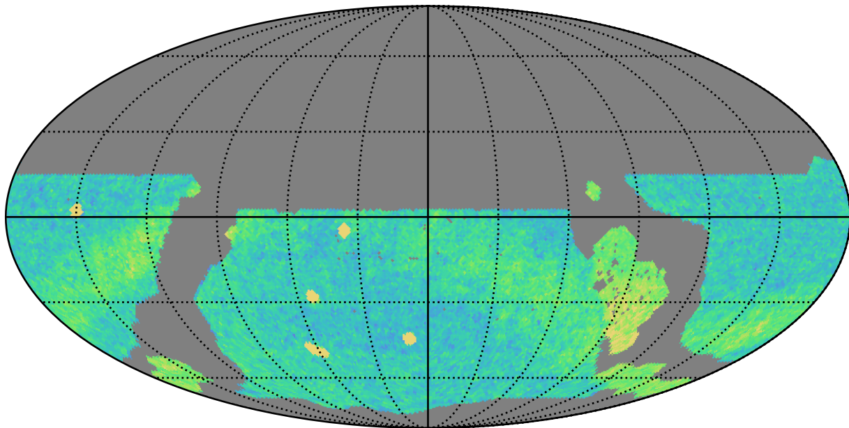
ddf_loaded_fl2_v3.4_10yrs WFD r band: NVisits
