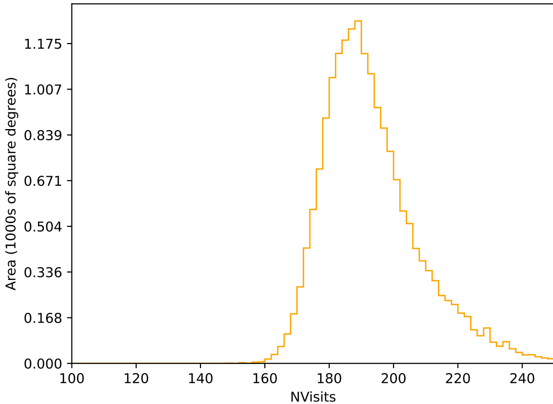
ddf_loaded_fl2_v3.4_10yrs WFD r band: NVisits
