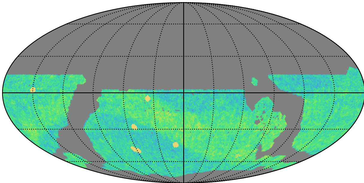
ddf_loaded_fl2_v3.4_10yrs WFD i band: NVisits
