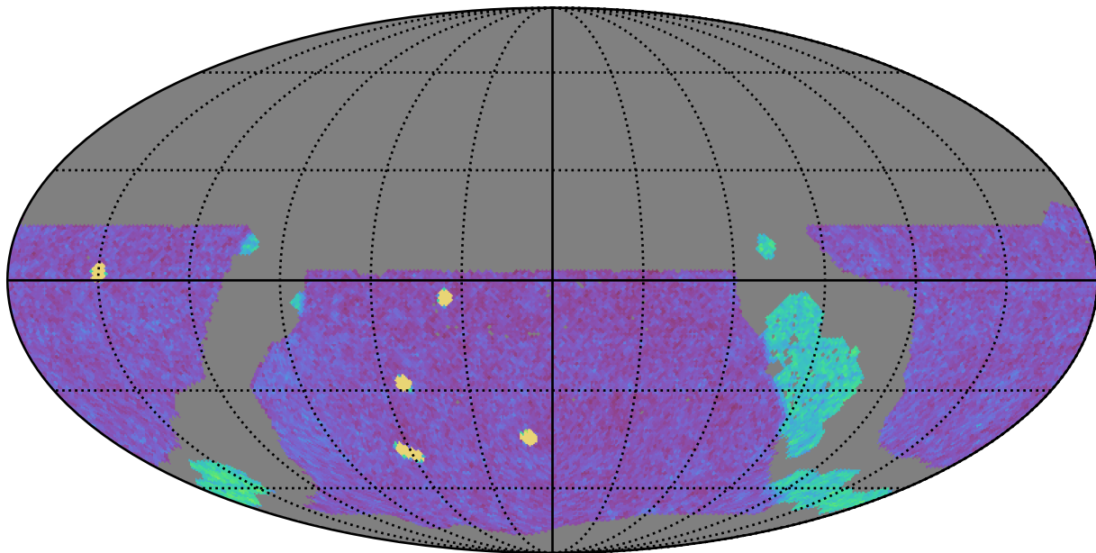
ddf_loaded_fl2_v3.4_10yrs WFD g band: NVisits
