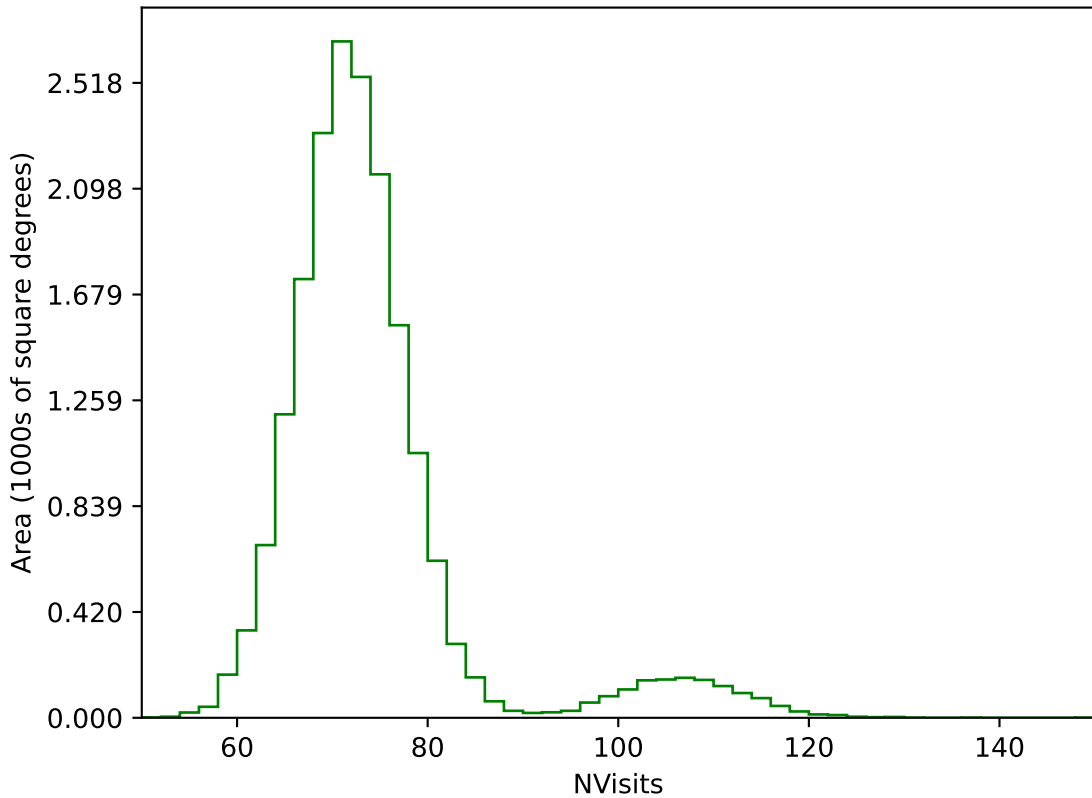
ddf_loaded_fl2_v3.4_10yrs WFD g band: NVisits
