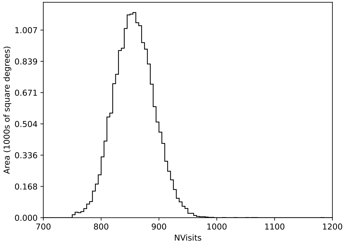
ddf_loaded_fl2_v3.4_10yrs WFD all bands: NVisits
