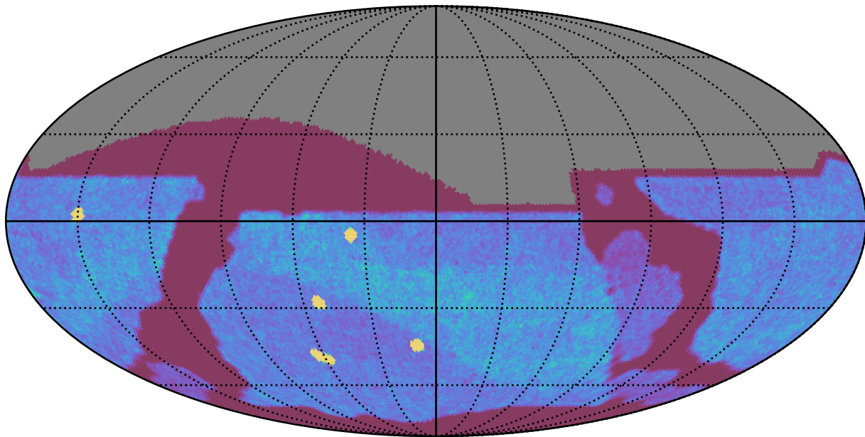
ddf_loaded_fl2_v3.4_10yrs All sky z band: NVisits
