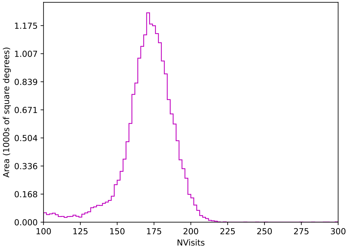
ddf_loaded_fl2_v3.4_10yrs All sky z band: NVisits
