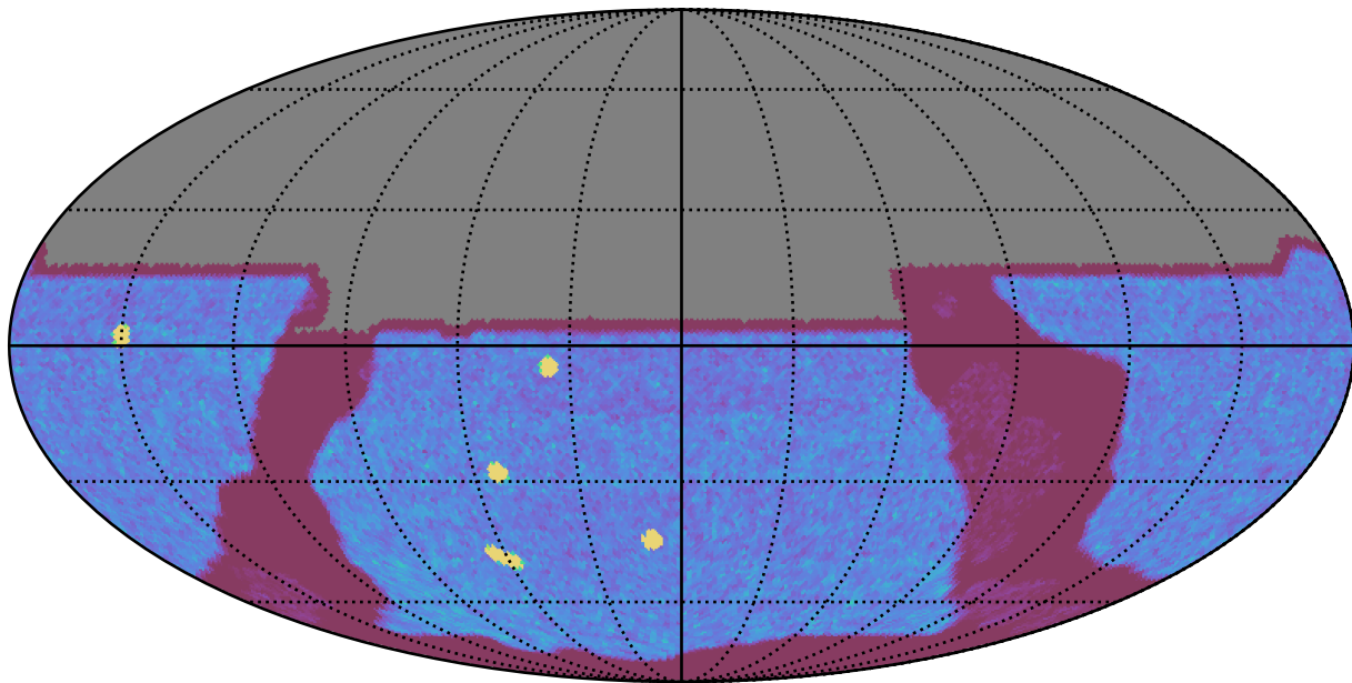
ddf_loaded_fl2_v3.4_10yrs All sky y band: NVisits
