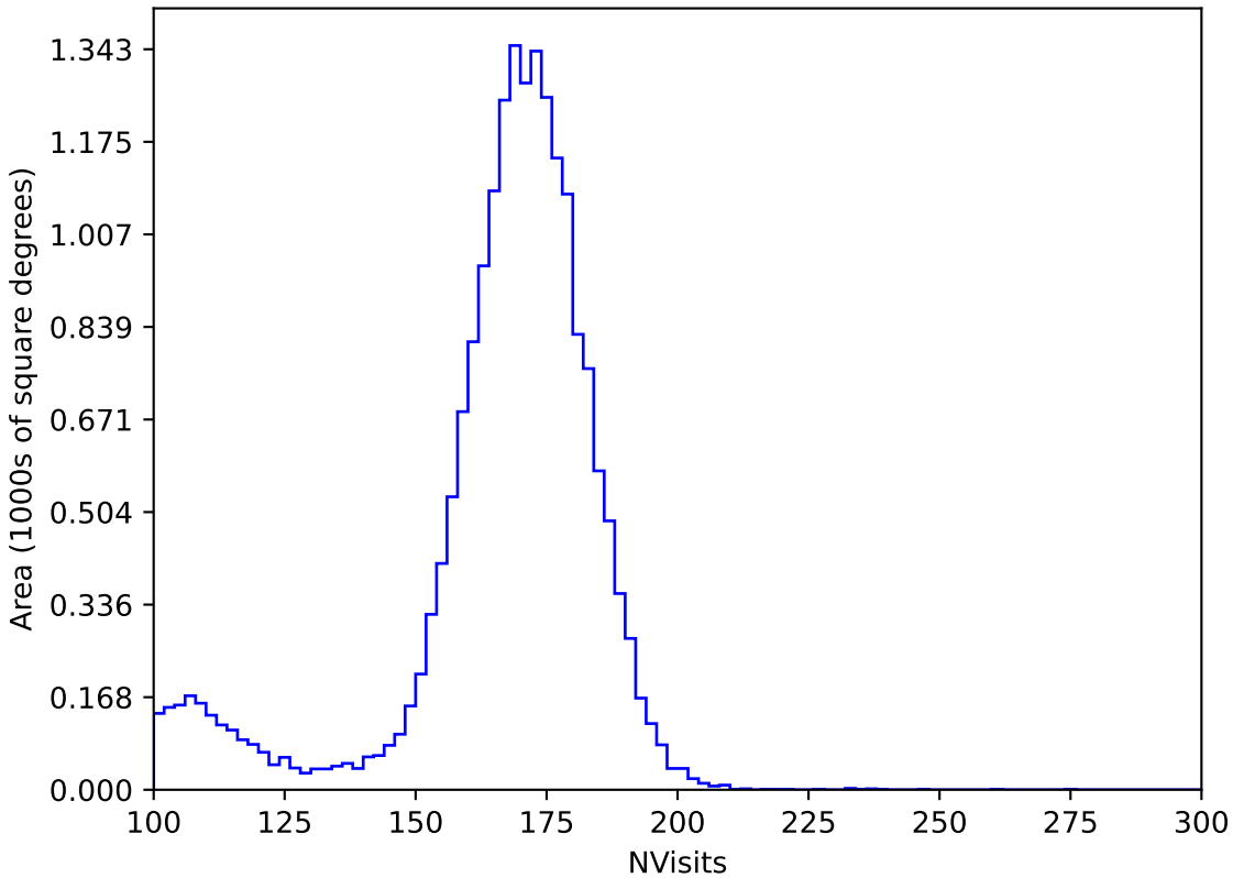
ddf_loaded_fl2_v3.4_10yrs All sky y band: NVisits
