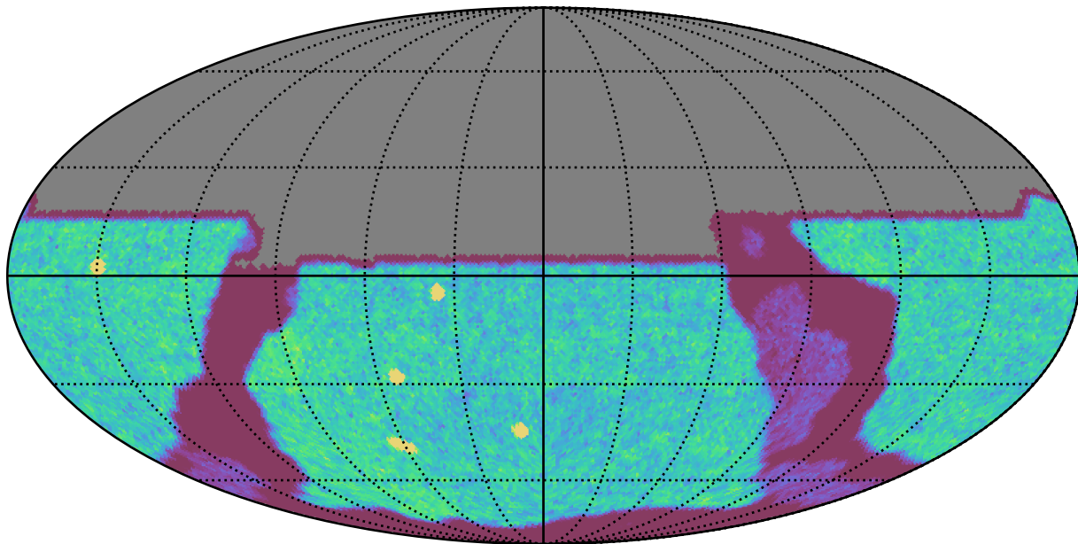
ddf_loaded_fl2_v3.4_10yrs All sky u band: NVisits
